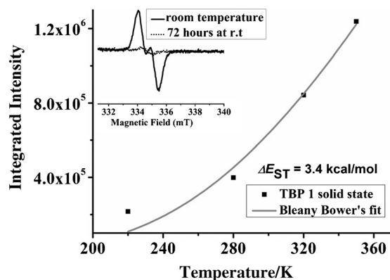
Figure 3. The change in EPR signal intensity with temperature (■) and the Bleany–Bower's fit (—). Inset: EPR spectra of TBP 1 in toluene solution at room temperature and after 72 h.
